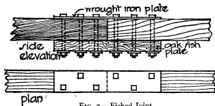
FIG. 2.—Fished Joint.
