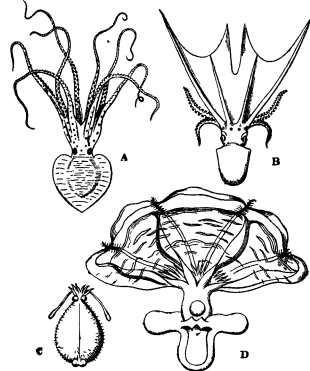
FIG. 38.—Octopodous Cephalopods.
