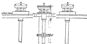
FIG. 2.—Elevation looking aft
