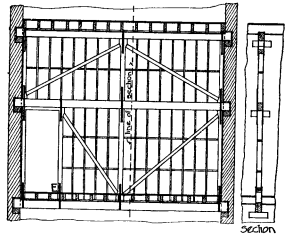
FIG. 33.—King Post Trussed Partition.
