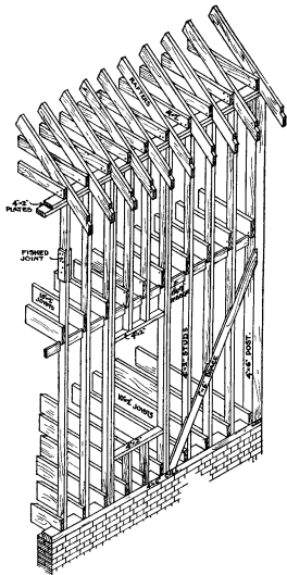
FIG. 36.—Balloon Frame.
