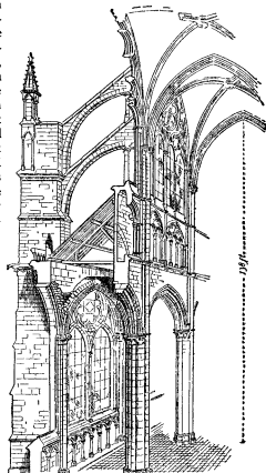
FIG. 8.—Perspective of Amiens Cathedral.
