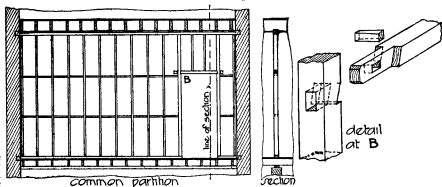
FIG. 30.—Common Partition.
