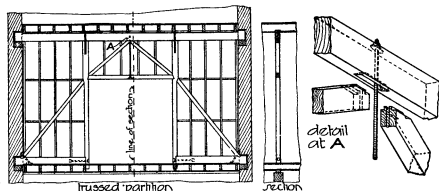
FIG. 31.—Trussed Partition.
